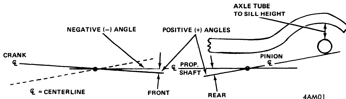
FRONT & REAR UNIVERSAL JOINT ANGLES
