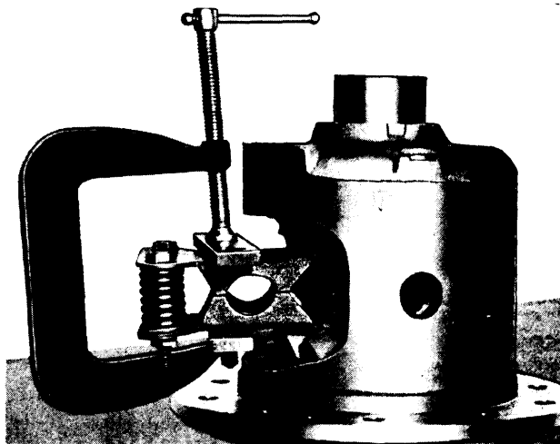
REMOVING PRELOAD SPRING PACK
