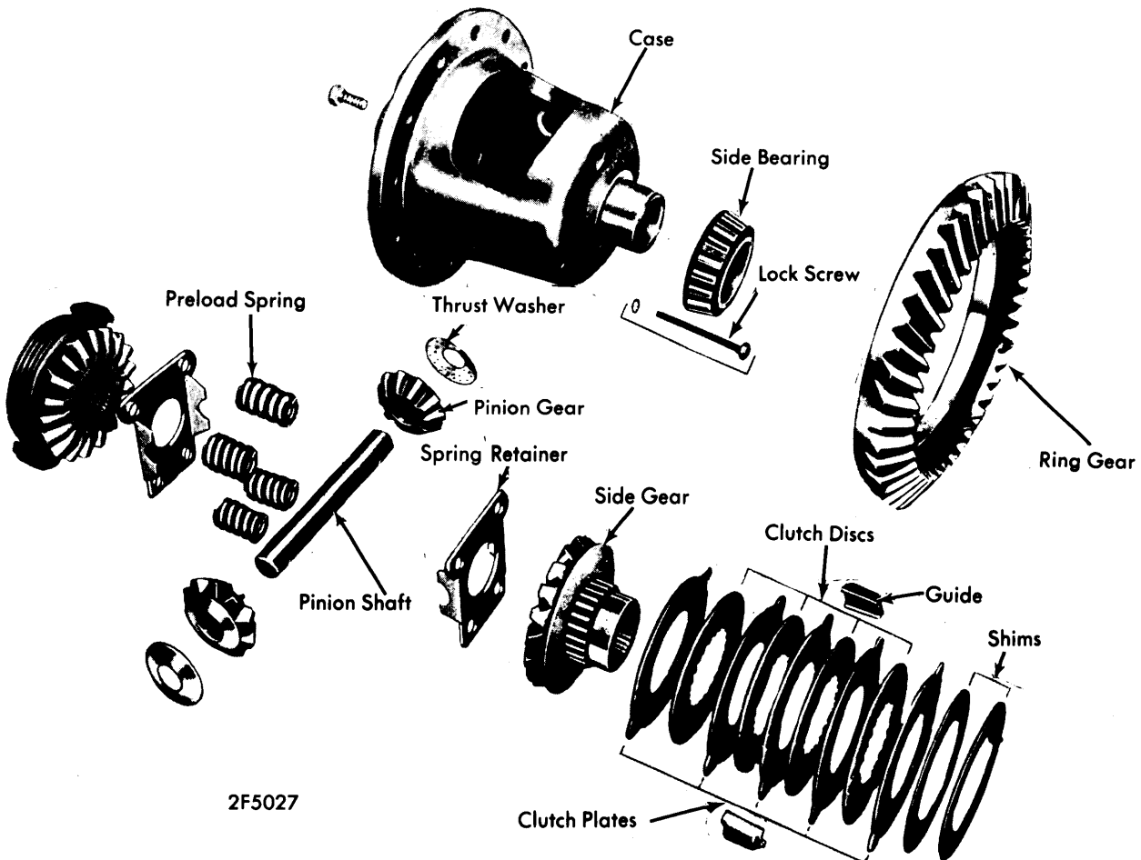
EATON BUILT POSITRACTION UNIT
