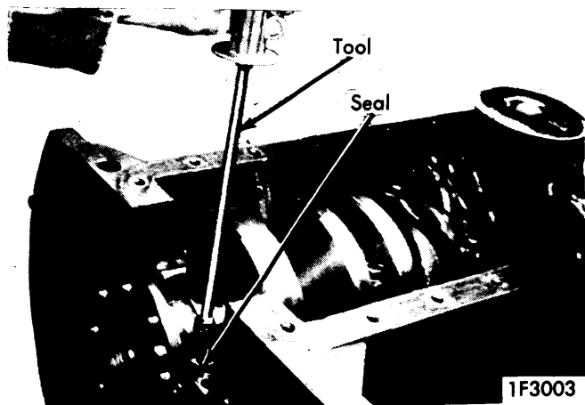
1F3003 USING TOOL ON UPPER REAR MAIN OIL SEAL
