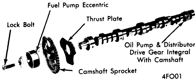
318" & 360" ENGINE CAMSHAFT
