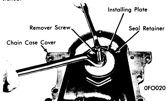
OFO020 INSTALLING FRONT COVER OIL SEAL
