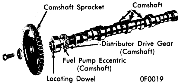
400" & 440" ENGINE CAMSHAFT
