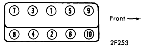
318" & 360" CYLINDER HEAD TIGHTENING SEQUENCE
