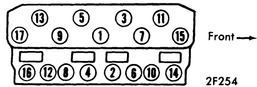
400" & 440" CYLINDER HEAD TIGHTENING SEQUENCE
