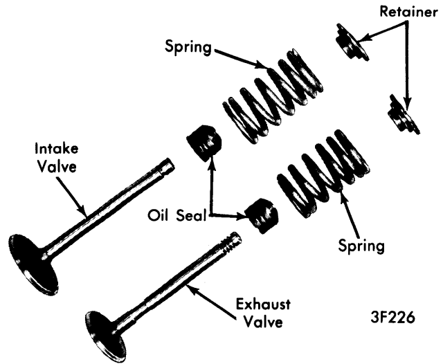
VALVE ASSEMBLIES
