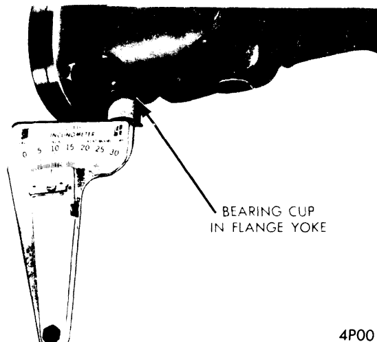
CHECKING UNIVERSAL JOINT ANGLE (TYPICAL)
