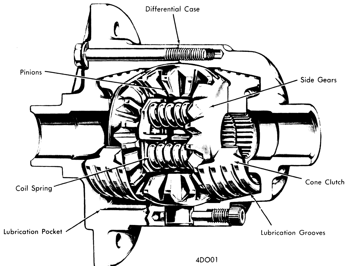
CHRYSLER CORP. SURE-GRIP DIFFERENTIAL ASSEMBLY
