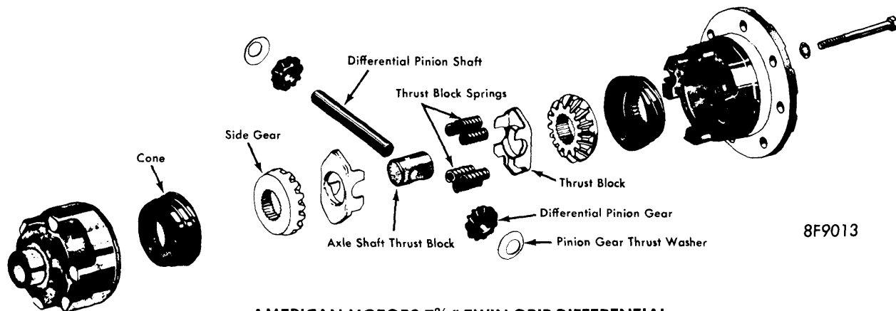
AMERICAN MOTORS 7 \frac{7}{16} " TWIN GRIP DIFFERENTIAL
