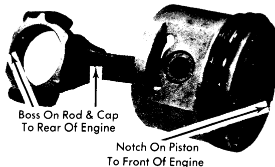
PISTON & ROD POSITION LEFT BANK - 455"
