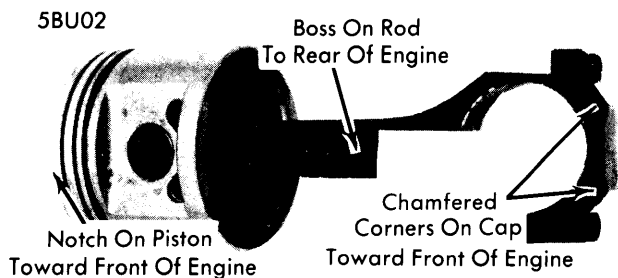
PISTON & ROD POSITION LEFT BANK - 350"
