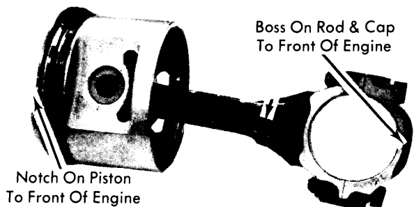
PISTON & ROD POSITION RIGHT BANK - 455"
