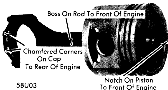
PISTON & ROD POSITION RIGHT BANK - 350"
