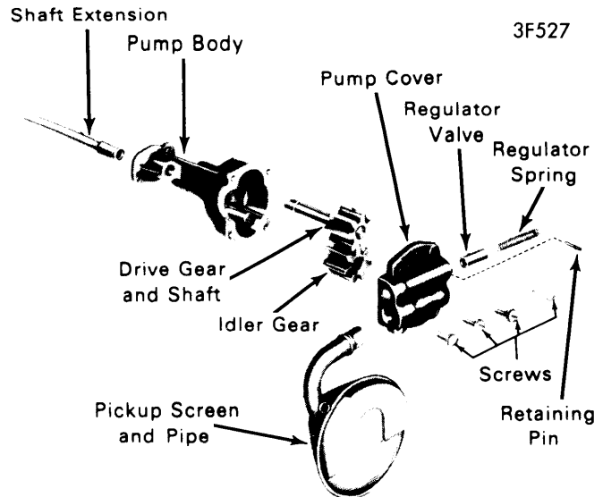
"SMALL V8" OIL PUMP ASSEMBLY
