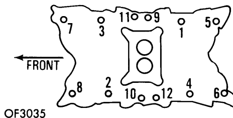
INTAKE MANIFOLD TIGHTENING SEQUENCE 351" M & 400"
