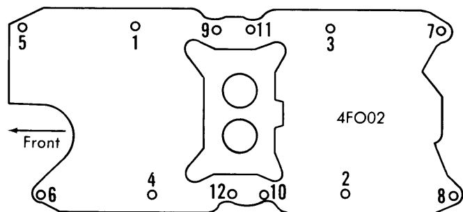
INTAKE MANIFOLD TIGHTENING SEQUENCE, 302"
