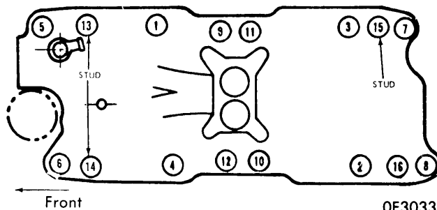
INTAKE MANIFOLD TIGHTENING SEQUENCE 351"W
