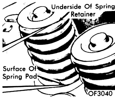
MEASURING VALVE SPRING INSTALLED HEIGHT
