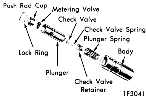
TYPE I LIFTER ASSEMBLY
