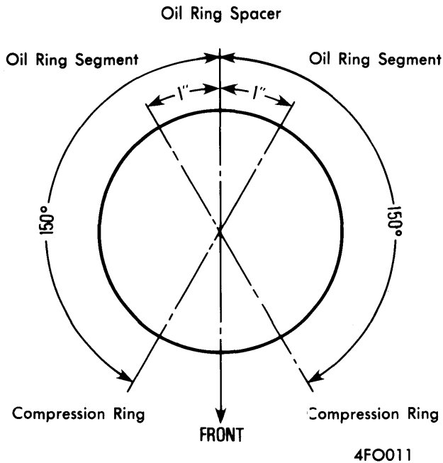
PISTON RING GAP SPACING
