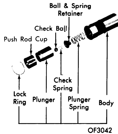
TYPE II LIFTER ASSEMBLY
