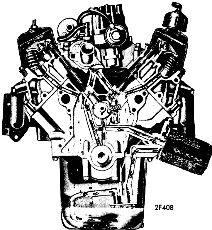
ENGINE OILING SYSTEM 302" & 351"W
