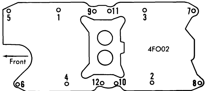
INTAKE MANIFOLD TIGHTENING SEQUENCE, 302"
