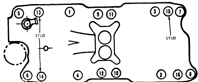
INTAKE MANIFOLD TIGHTENING SEQUENCE 351"W
