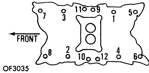
INTAKE MANIFOLD TIGHTENING SEQUENCE 351" C & 400"
