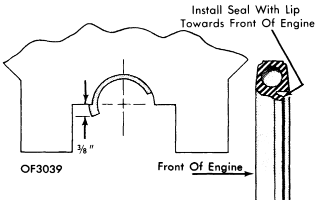
SPLIT LIP-TYPE REAR MAIN BEARING SEAL
