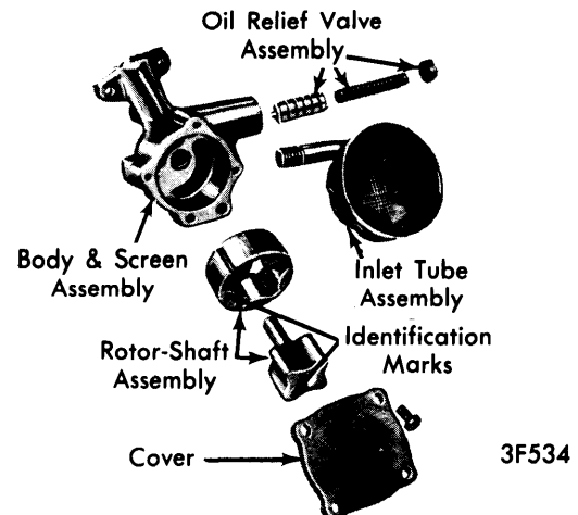
OIL PUMP ASSEMBLY (TYPICAL)
