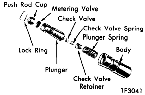
TYPE I LIFTER ASSEMBLY
