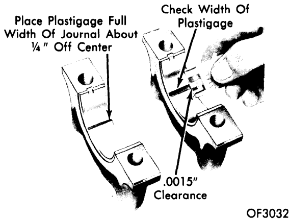
MEASURING BEARING CLEARANCE
