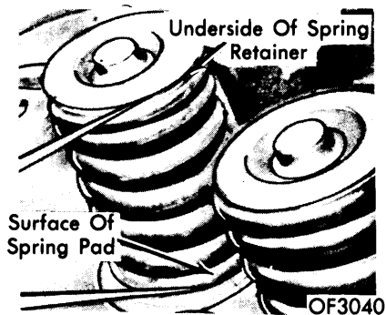
MEASURING VALVE SPRING INSTALLED HEIGHT
