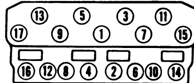
400" & 440" CYLINDER HEAD TIGHTENING SEQUENCE
