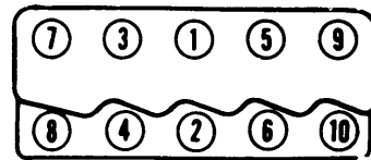
318" & 360" CYLINDER HEAD TIGHTENING SEQUENCE
