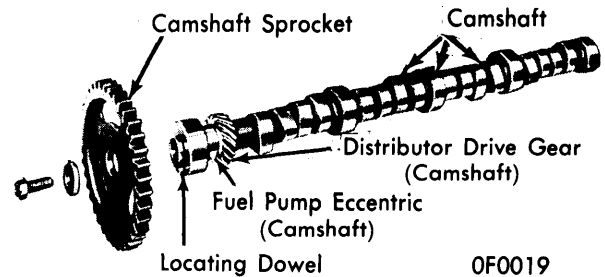
400" & 440" ENGINE CAMSHAFT
