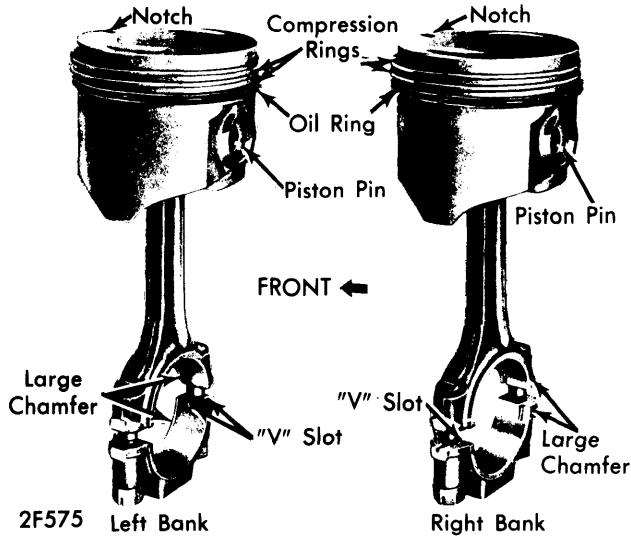
PISTON & ROD ASSEMBLY
