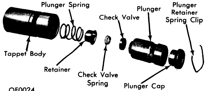
OF0024 HYDRAULIC VALVE LIFTER
