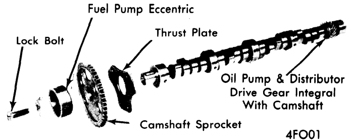
318" & 360" ENGINE CAMSHAFT
