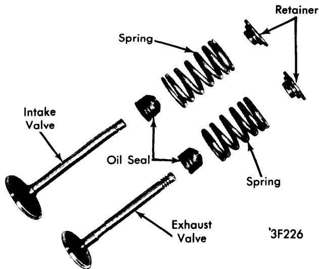
VALVE ASSEMBLIES
