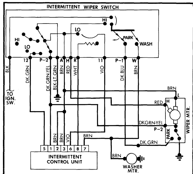
Fig. 3 Chrysler Corp. 2-Speed Concealed Intermittent Wiper Wiring Diagram (Aries, Reliant, LeBaron & 400)
