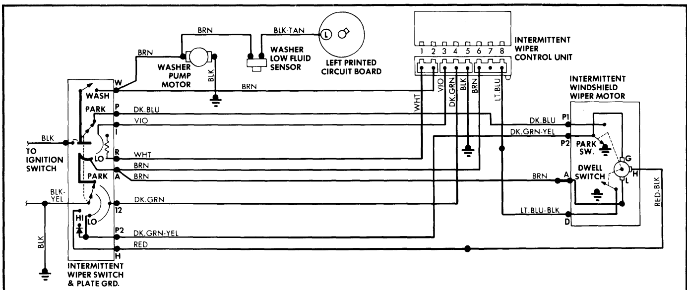
Fig. 4 Chrysler Corp. 2-Speed Concealed Intermittent Wiper Wiring Diagram (All Models Except Aries, Reliant, LeBaron & 400)
