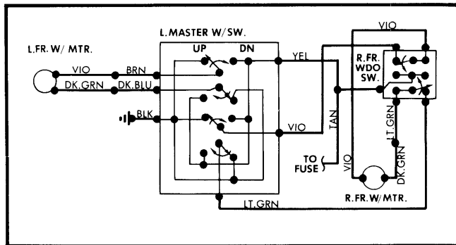
Fig. 4 Chrysler Corp. Power Window Wiring Diagram (Cordoba & Mirada)
