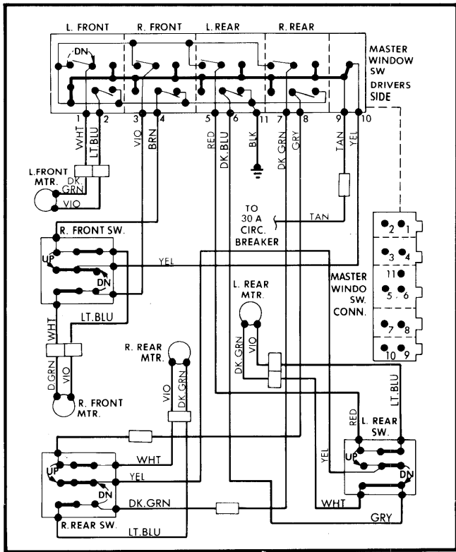
Fig. 3 Chrysler Corp. Power Window Wiring Diagram (Gran Fury, Newport & Diplomat)
