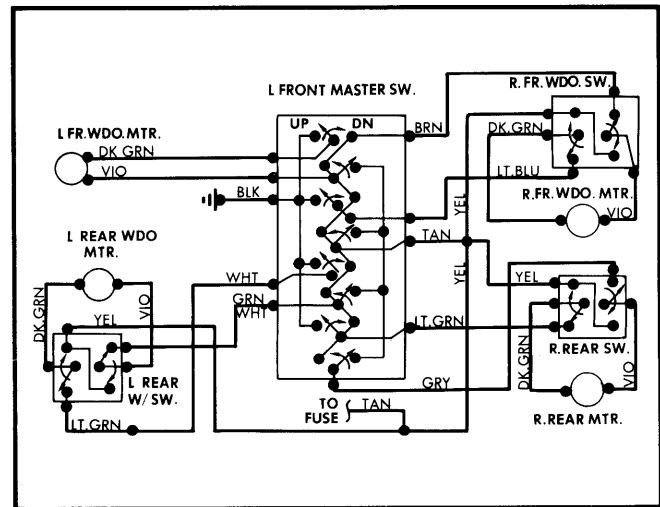
Fig. 6 Chrysler Corp. Power Window Wiring Diagram (Aries, Reliant, LeBaron & 400)
