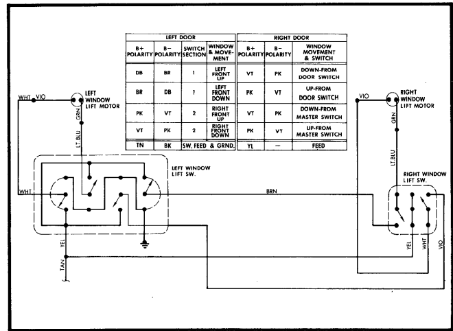
Fig. 5 Chrysler Corp. Power Window Wiring Diagram (Imperial)
