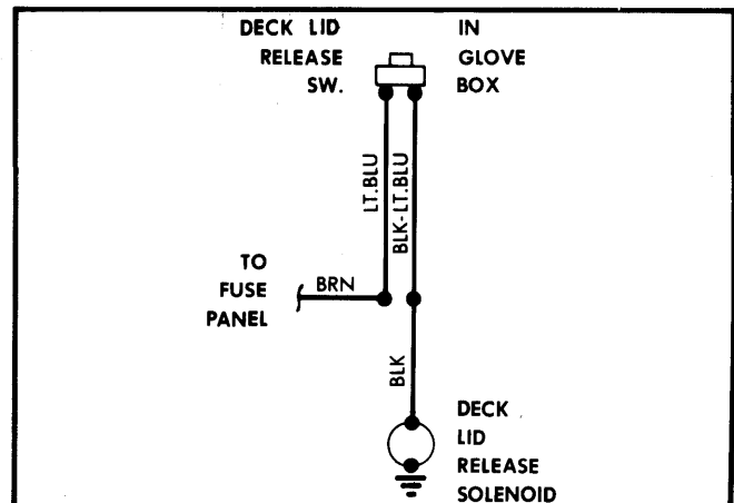
Fig. 2 Typical Chrysler Corp. Power Trunk and Tailgate Release Wiring Diagram
