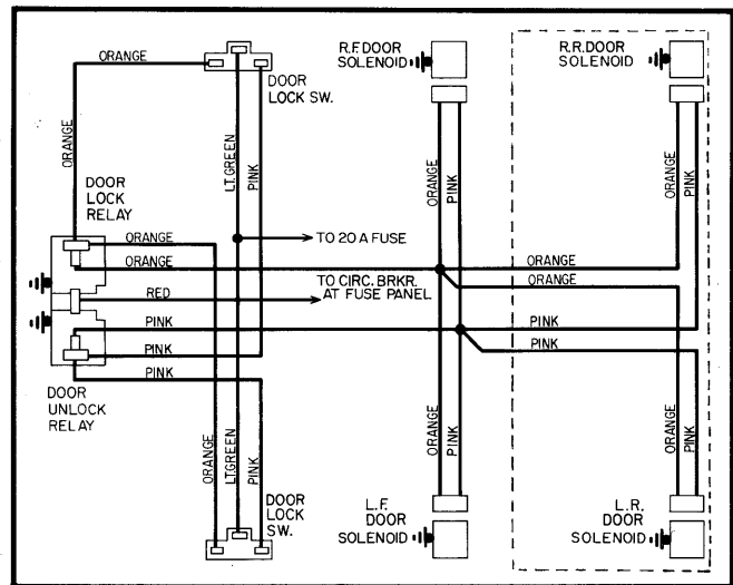
Fig. 1 Typical Chrysler Corp. Power Door Lock Wiring Diagram
