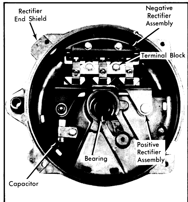
Fig. 4 View of Rectifier End Shield (114 Amp. Shown)
