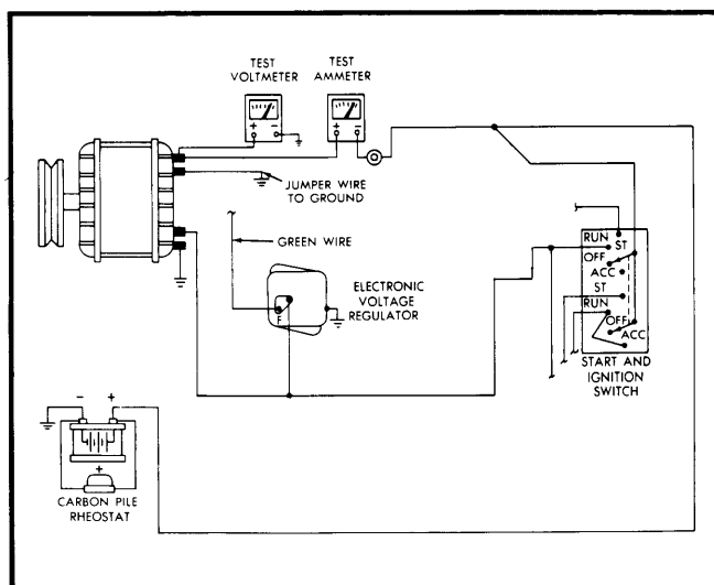
Fig. 2 Diagram Showing Meter Connections for Alternator Current Output Test
