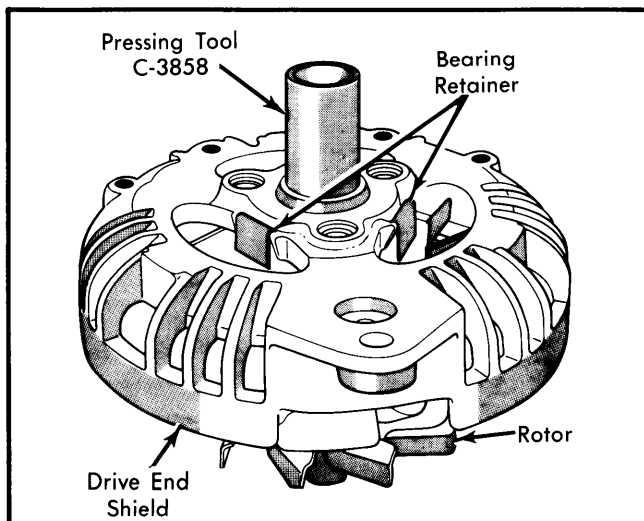
Fig. 3 Installing Drive End Shield Bearing (All Except 114 Amp. Shown)
