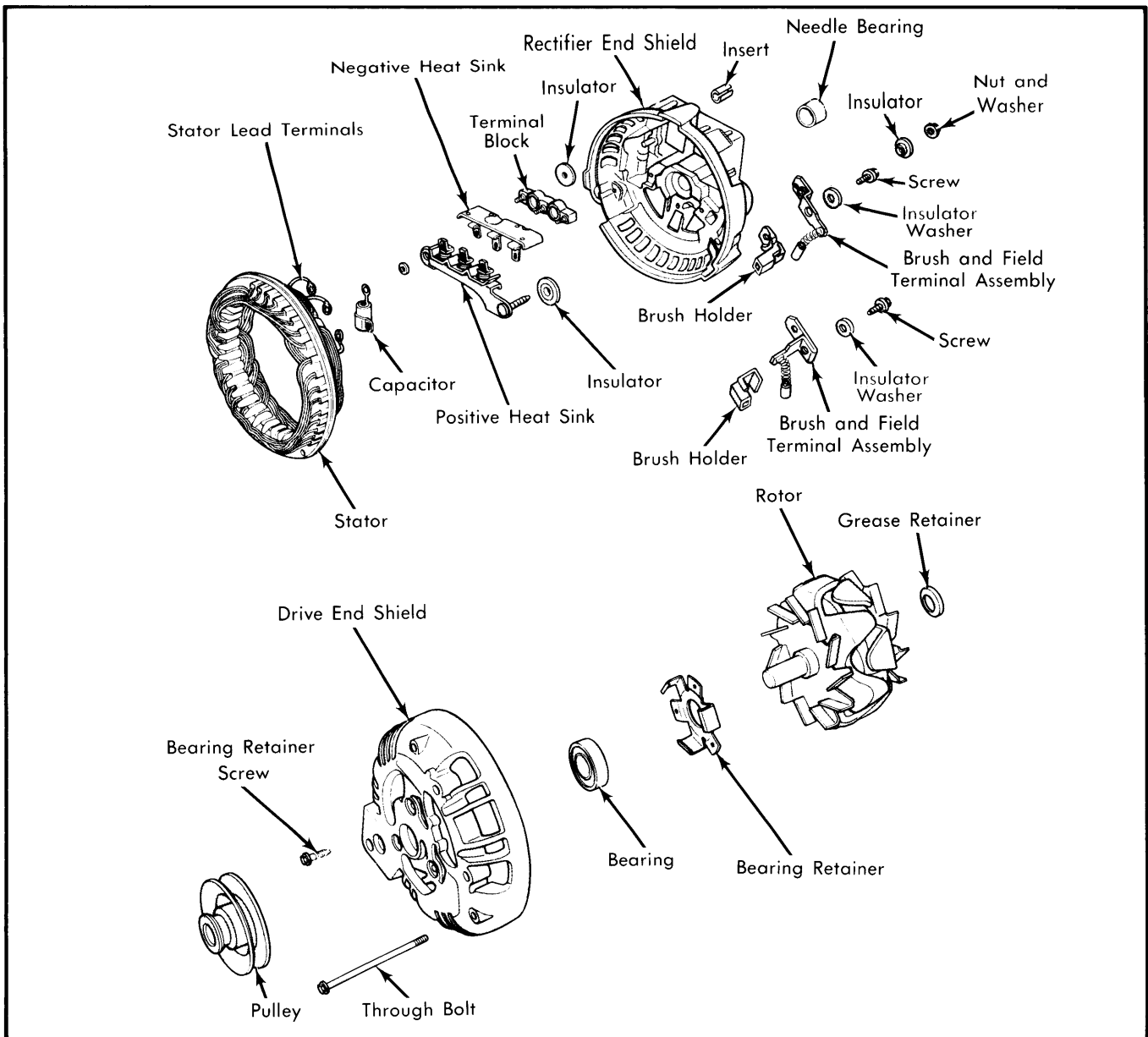
Fig. 6 Exploded View of Chrysler Corp. Alternator (60 Amp. Shown; Other Models Similar)
