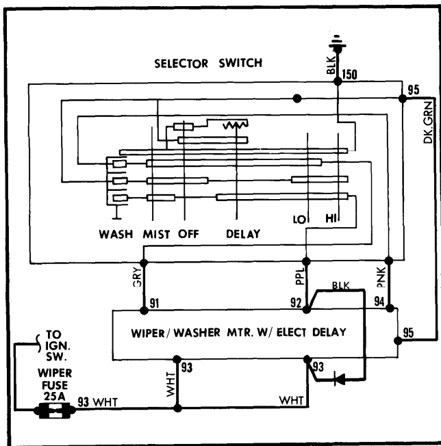
Fig. 1 Multiplex Wiper Wiring Diagram
