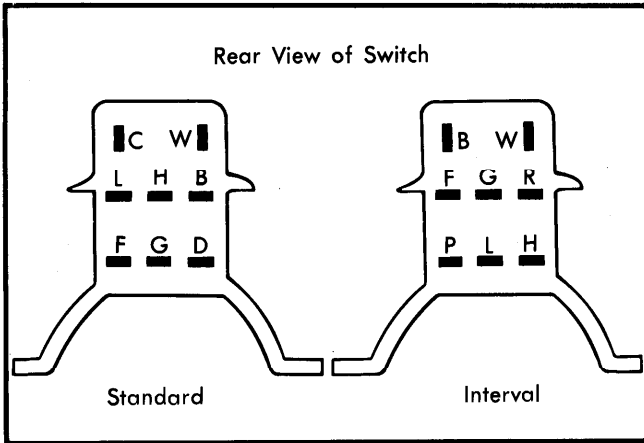
Fig. 3 Wiper Switch Continuity Test Terminal Locations
