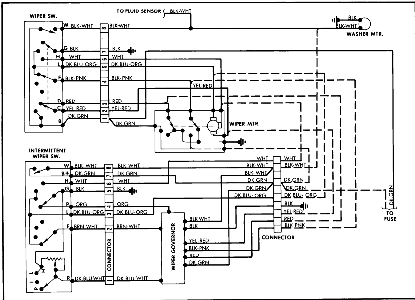
Fig. 4 Concealed Wiper System Wiring Diagram (Ford, Mercury, Lincoln Town Car & Mark VI)
