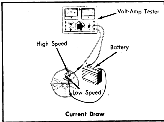
Fig. 1 Motor Current Draw Test Connections
