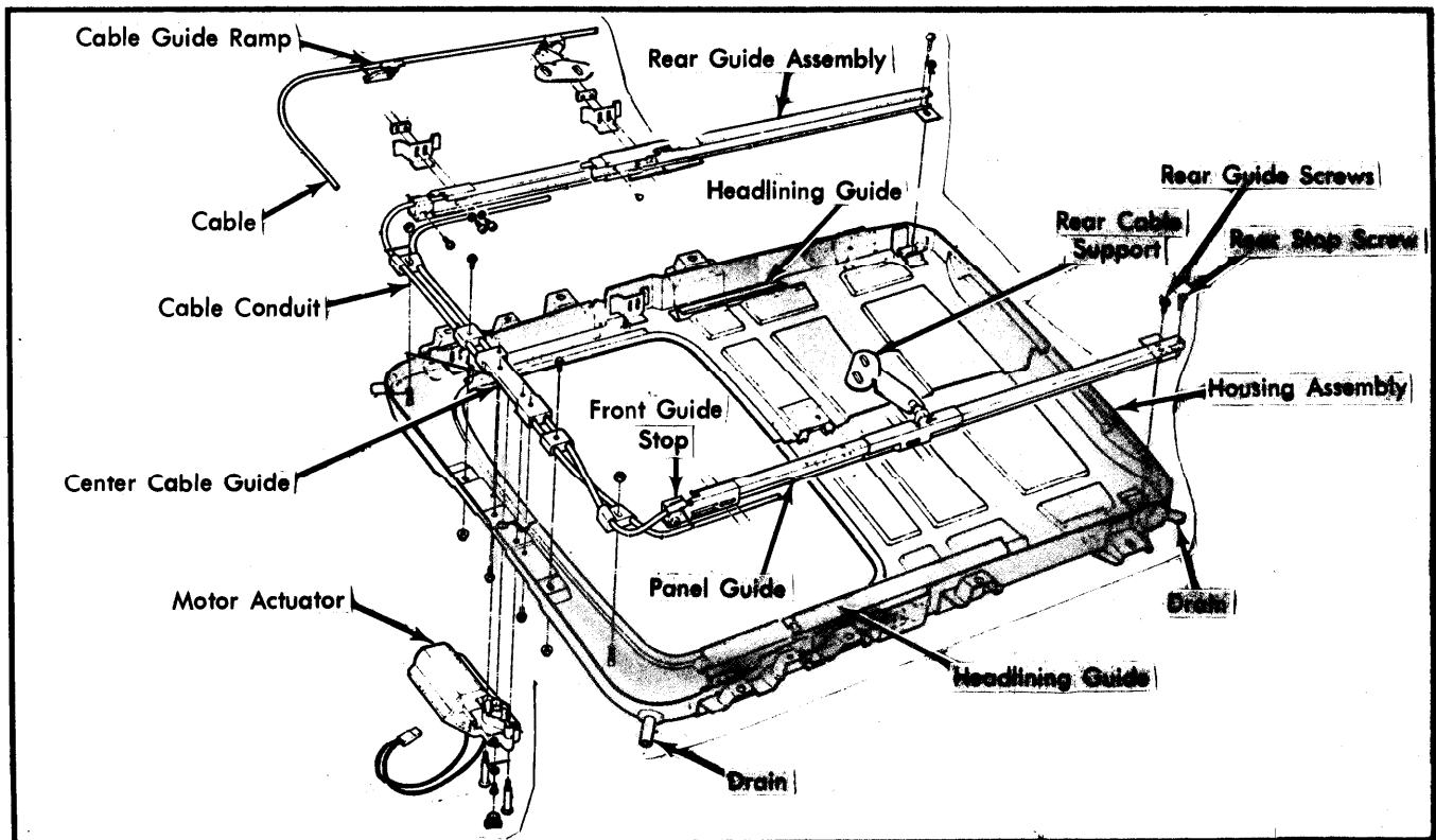
Fig. 1 Exploded View of Sun and Moon Roof Assembly
