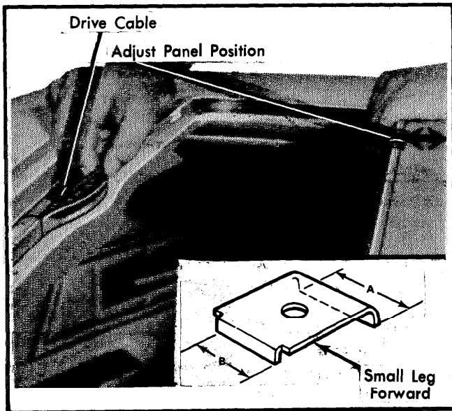
Fig. 1 Roof Panel Horizontal Adjustment
