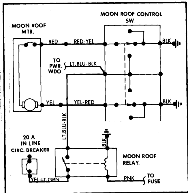
Fig. 2 Power Roof Panel Wiring Diagram
