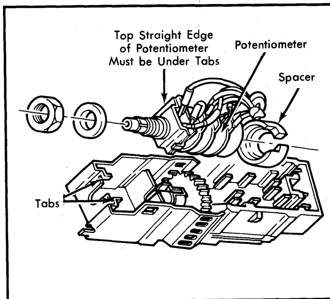
Fig. 1 Headlight Switch Assembly (Ford, Mercury, Lincoln & Mark VI Other Models Similar)
