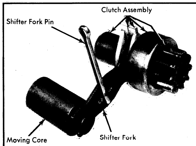
Fig. 2 Shift Fork and Clutch Assembly
