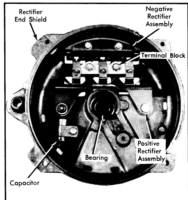
Fig. 4 View of Rectifier End Shield (100 Amp. Shown)
