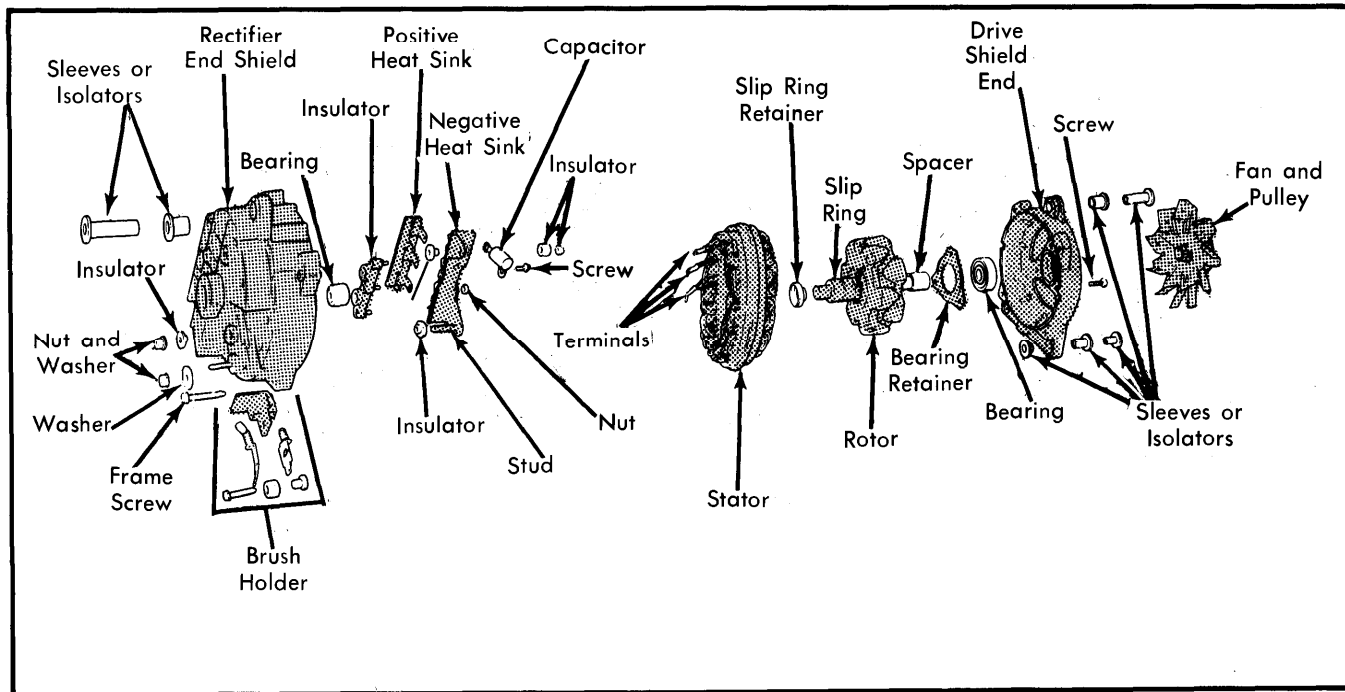
Fig. 7 Exploded View of Chrysler Corp. Alternator (100 Amp.)
