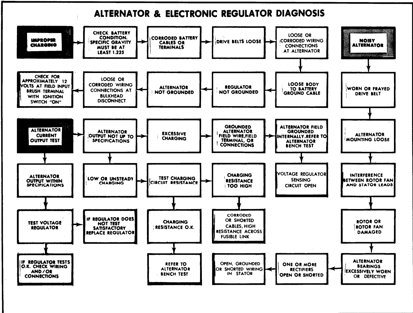
Fig. 5 Charging Circuit Service Diagnosis Guide for All Chrysler Corp. Vehicles
