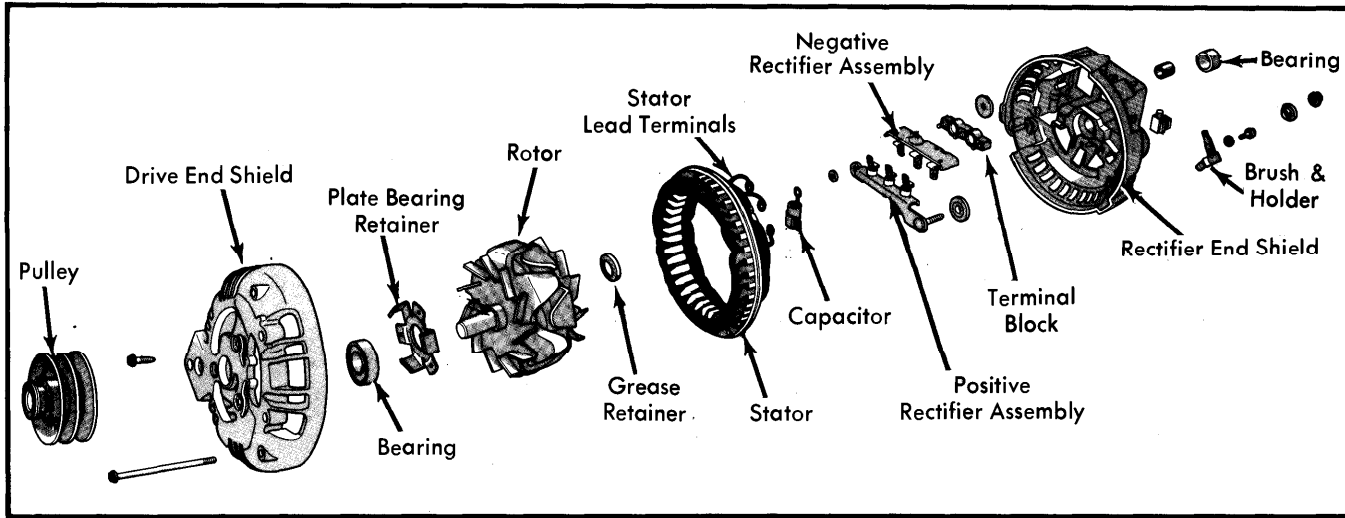
Fig. 6 Exploded View of Chrysler Corp. Alternator (Except 100 Amp.)
