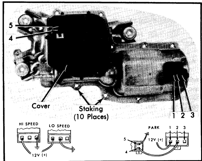
Fig. 2 Integral Motor Wiring Connections
