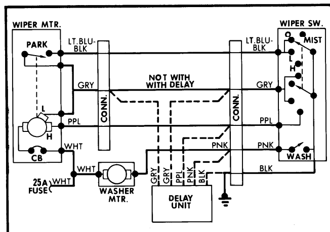
Fig. 1 General Motors Integral Wiper Wiring Diagram Citation, Omega, Phoenix, Skylark Standard and Intermittent
