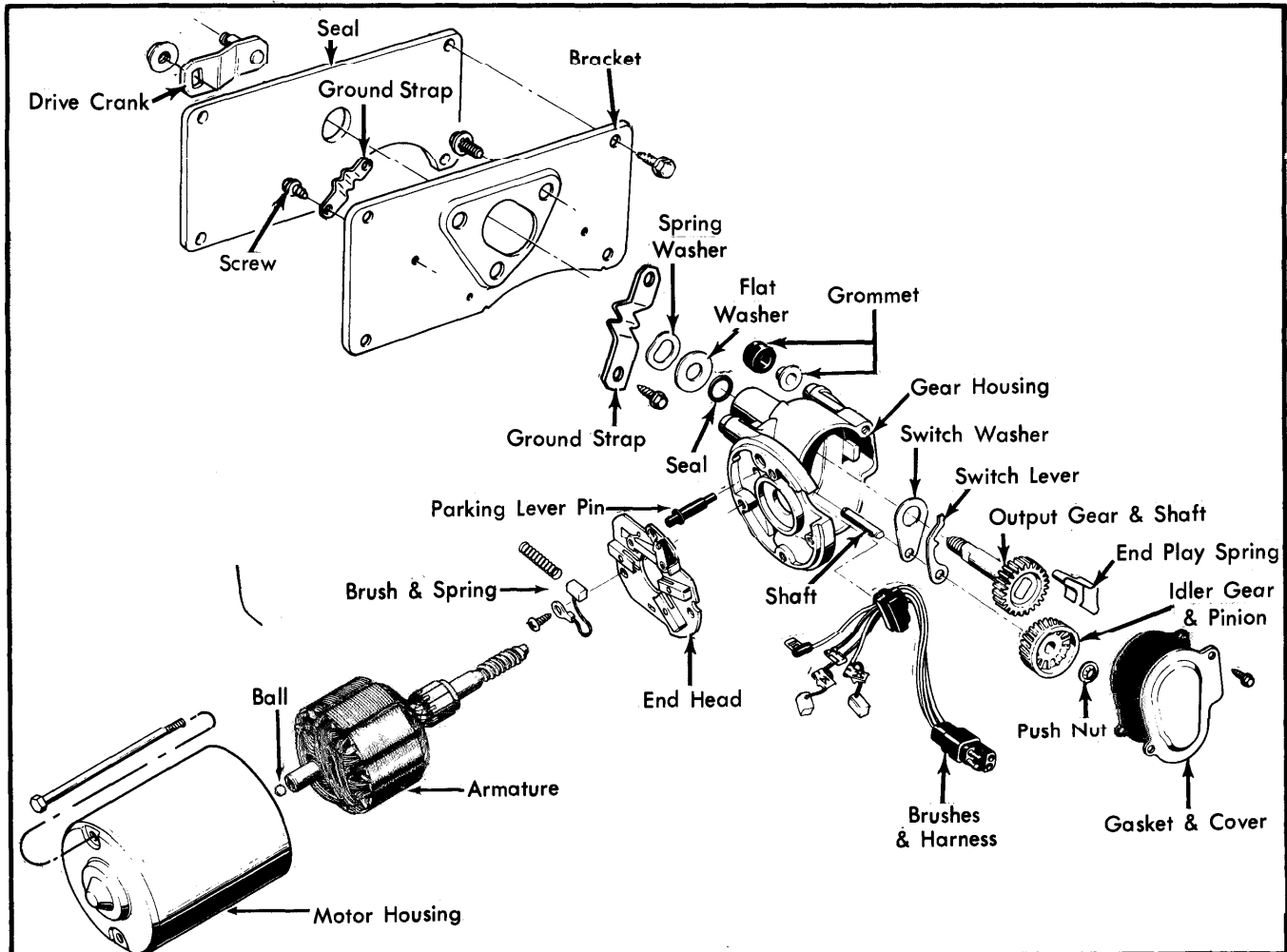
Fig. 2 Exploded View of AMC Wiper Motor & Transmission
