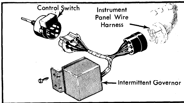
Fig. 3 Windshield Wiper Instrument Panel Wiring Showing Intermittent Governor
