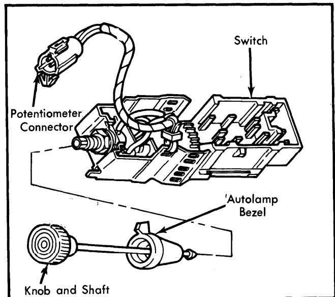
Fig. 2 Autolamp Headlight Switch Assembly Ford, Mercury, Cougar XR-7 (Thunderbird Similar)
