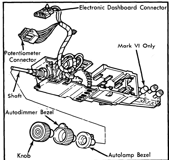
Fig. 1 Autolamp Headlight Switch Assembly Continental & Mark VI
