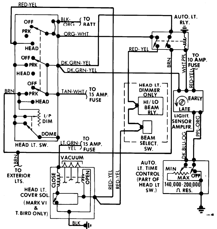
Fig. 4 Autolamp Wiring Diagram (All Models)
