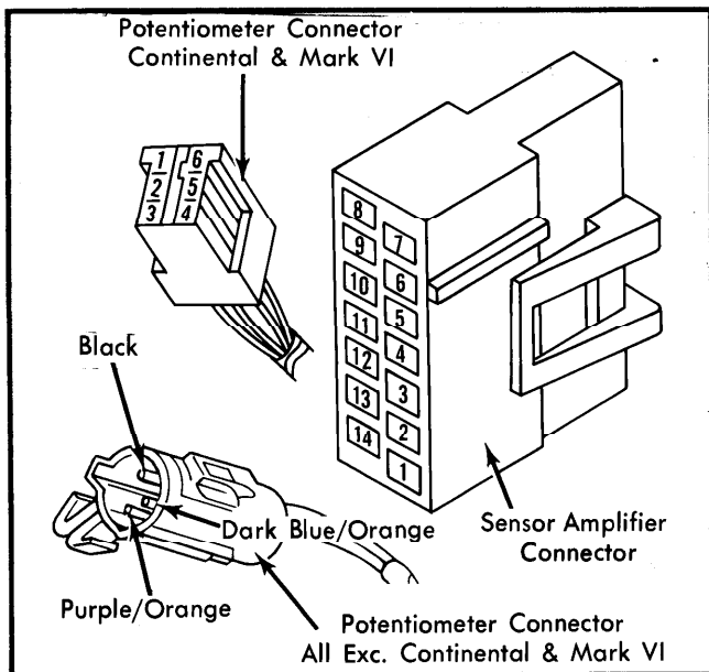
Fig. 3 Autolamp Circuit Connectors Terminal Identification
