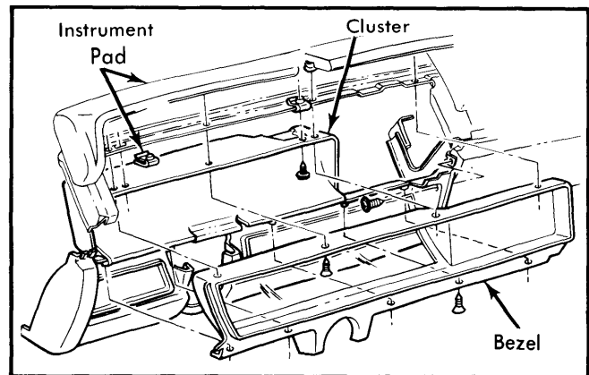
Fig. 1 Exploded View of Standard One Piece Instrument Panel Cluster — Monza and Sunbird
