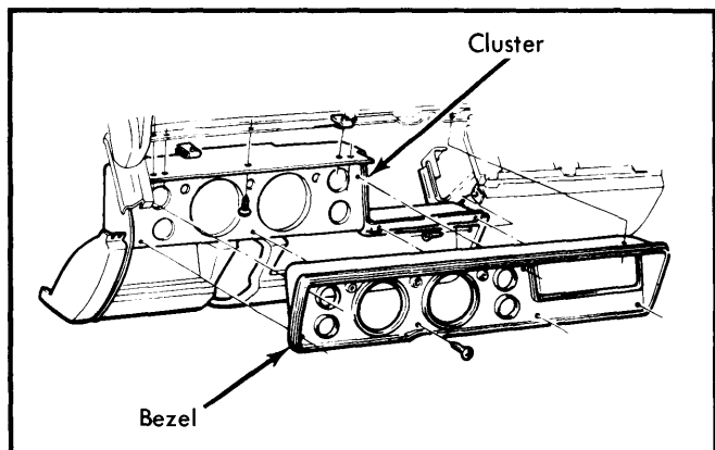
Fig. 2 Exploded View of GT Instrument Panel Cluster — Monza Sport Coupe and Sunbird Sport
