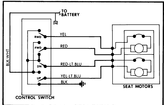
Fig. 2 Granada, Monarch, Fairmont & Zephyr 4-Way Power Seat Wiring Diagram (Versailles Similar)
