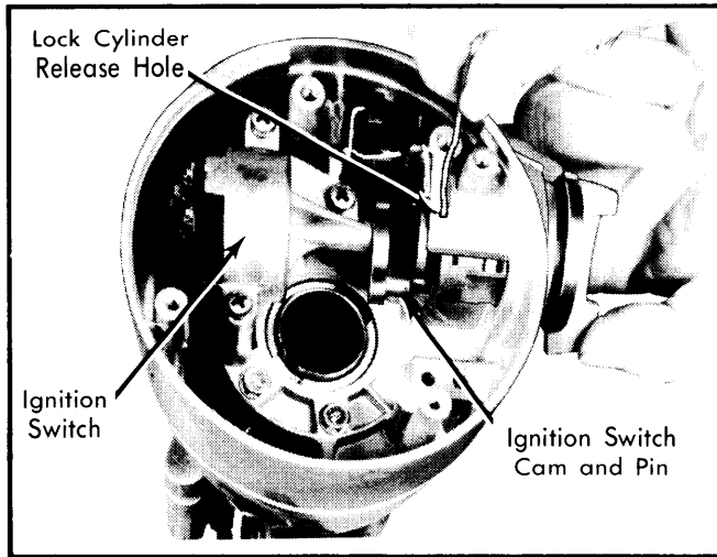
Fig. 4 Depressing Lock Cylinder Retaining Tab Chrysler Corp. Models with Standard Steering Columns
