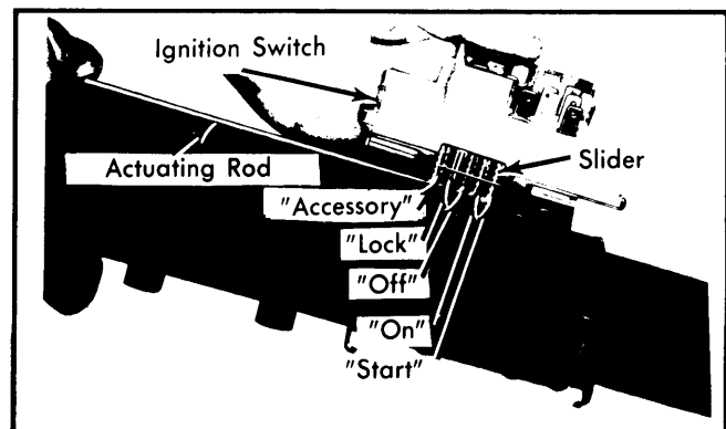
Fig. 5 Rod Actuated Ignition Switch Common to All Models
