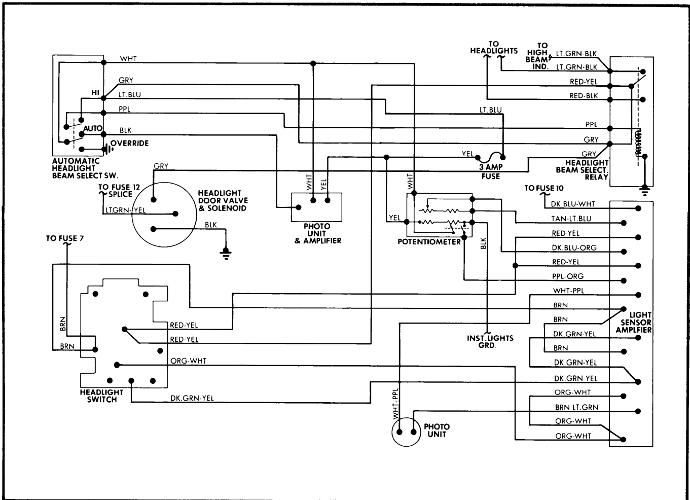
Fig. 3 Continental Mark V Autolamp Wiring Diagram
