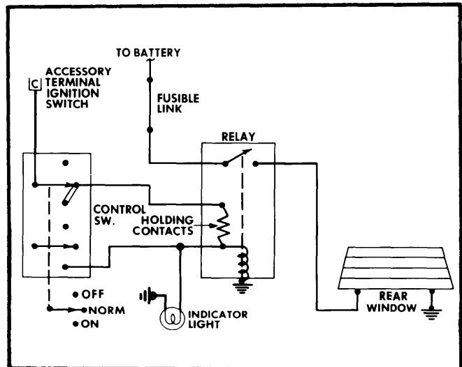
Fig. 3 Heated Rear Window Wiring Diagram Lincoln Continental
