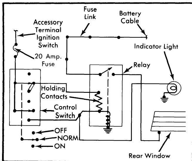
Fig. 1 Heated Rear Window Wiring Diagram (All Except Lincoln Continental)
