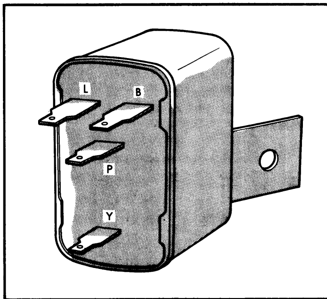
Fig. 1 Timer Relay Connections St. Regis, Newport & New Yorker
