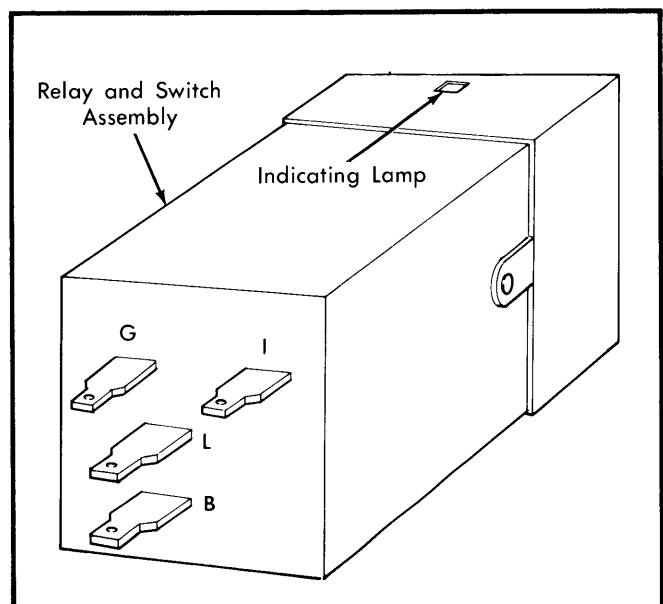
Fig. 3 Timer Relay Connections Except St. Regis, Newport, New Yorker, Horizon & Omni
