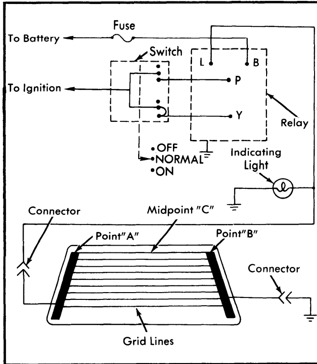
Fig. 4 Chrysler Heated Rear Window Wiring Diagram Except St. Regis, Newport, New Yorker, Horizon & Omni
