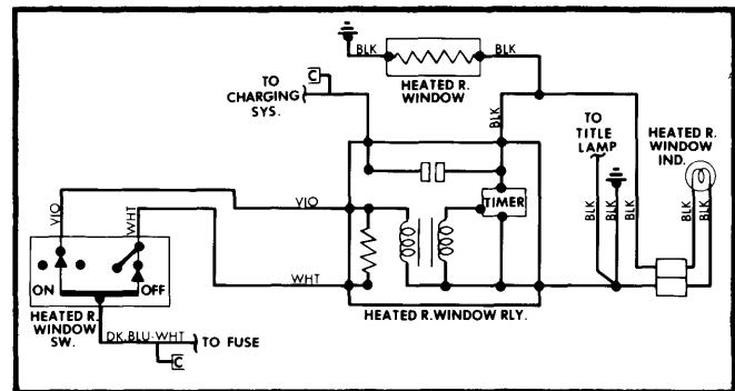
Fig. 6 Horizon & Omni Rear Window Wiring Diagram
