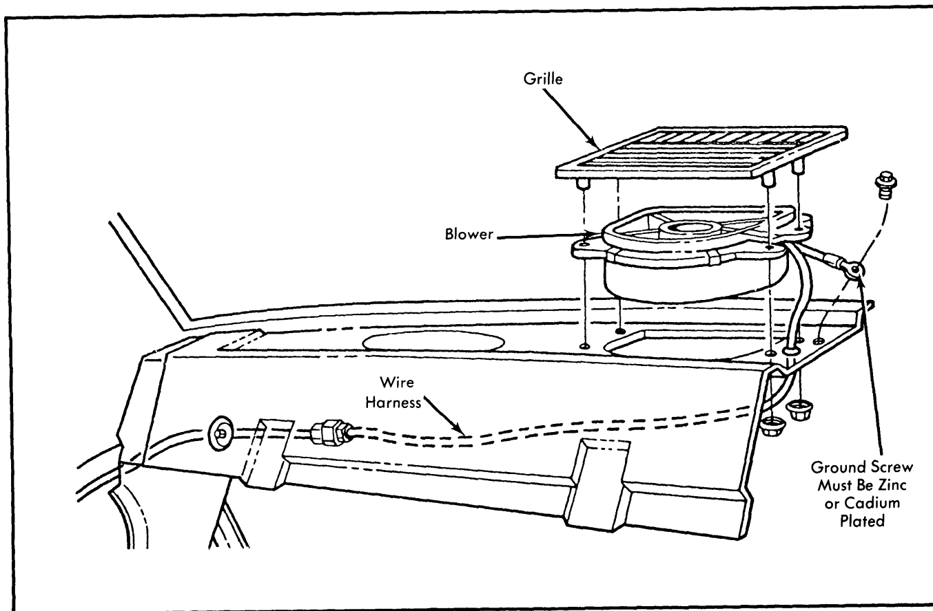
Fig. 2 Component Layout of Rear Window Defogger Fan System (Ford Motor Co. Shown)
