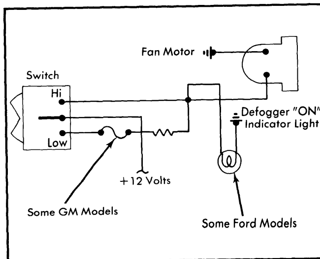
Fig. 1 Wiring Diagram of Rear Window Defogger Fan Circuit with Resistor or Resistance Wire in Circuit
