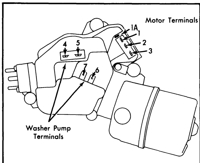
Fig. 2 Modified Pulse Wiper Motor Terminals
