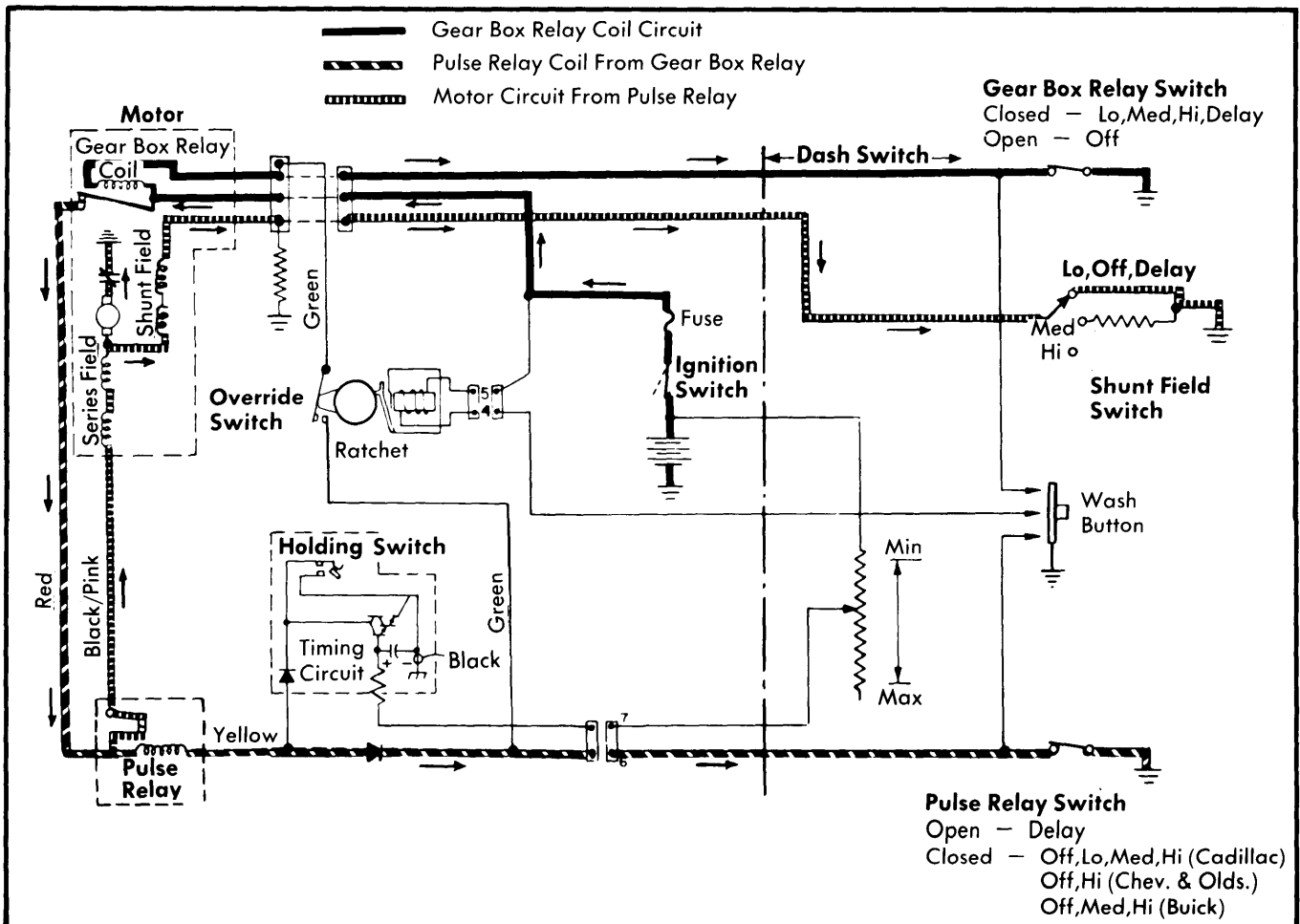
Fig. 1 Modified Pulse Wiper Wiring Diagram (Cadillac "Lo" Speed Shown)
