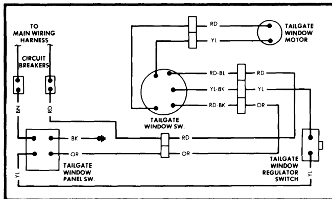
Fig. 1 Power Tailgate Window Wiring Diagram American Motors
