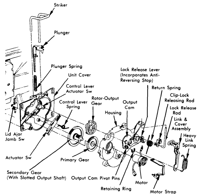
Fig. 2 Cadillac Electric Closing Unit Components
