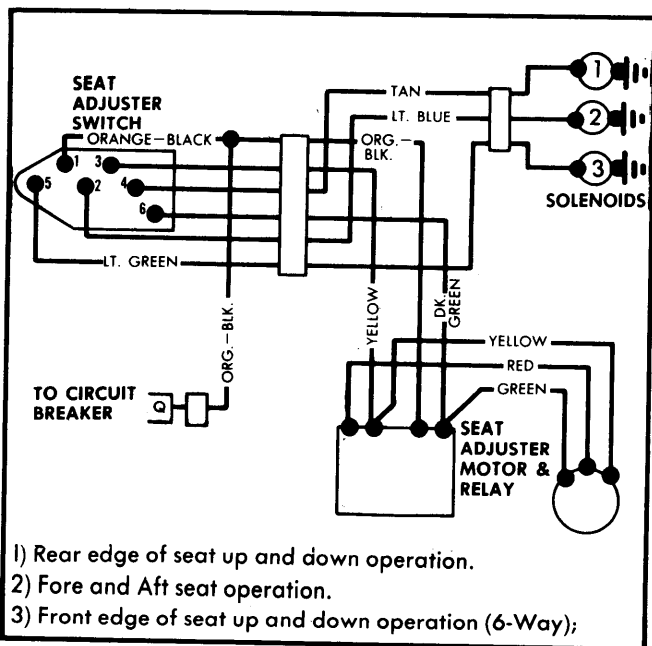
Fig. 2 6-Way General Motors Power Seat Wiring Diagram (Exc. C-69 Style Cadillac)
