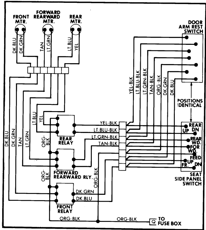
Fig. 3 6-Way General Motors Power Seat Wiring Diagram (Cadillac C-69 Styles Only)
