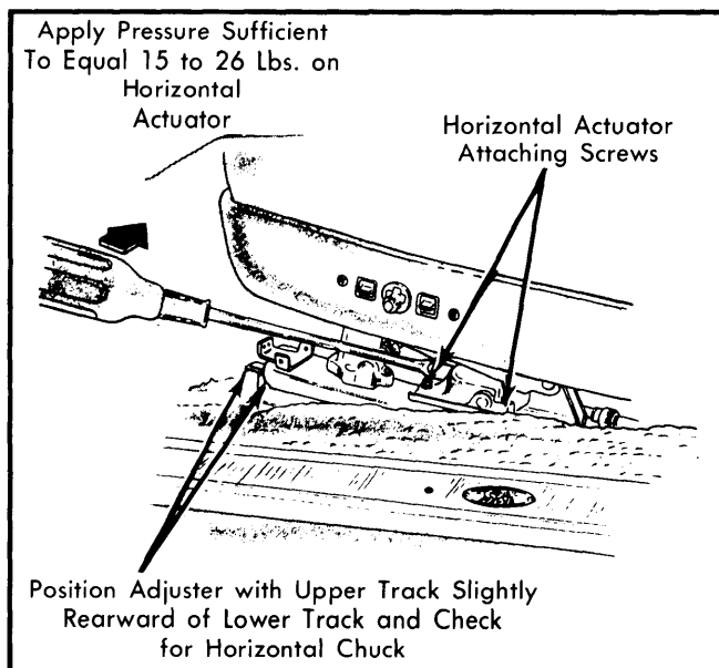
Fig. 5 Horizontal Actuator Adjustment
