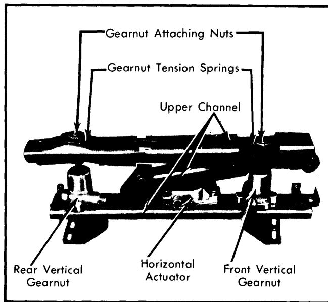
Fig. 6 6-Way Seat Adjuster Mechanism
