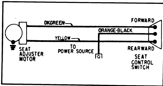
Fig. 1 2-Way General Motors Power Seat Wiring Diagram
