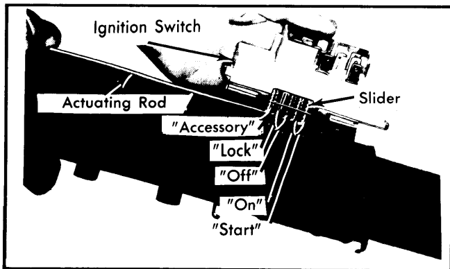
Fig. 5 Rod Actuated Ignition Switch Common to All Models
