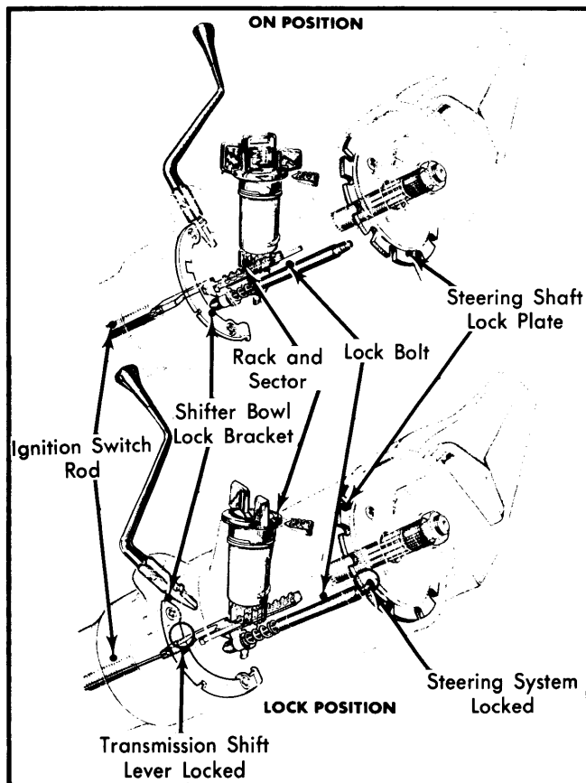
Fig. 1 Steering Column Locking Mechanism Except Chrysler Corp. Standard Steering Column
