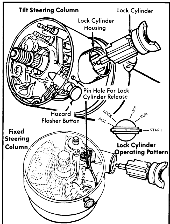
Fig. 6 Ford Motor Co. Lock Cylinder Assembly Showing Lock Cylinder Release Pin Hole
