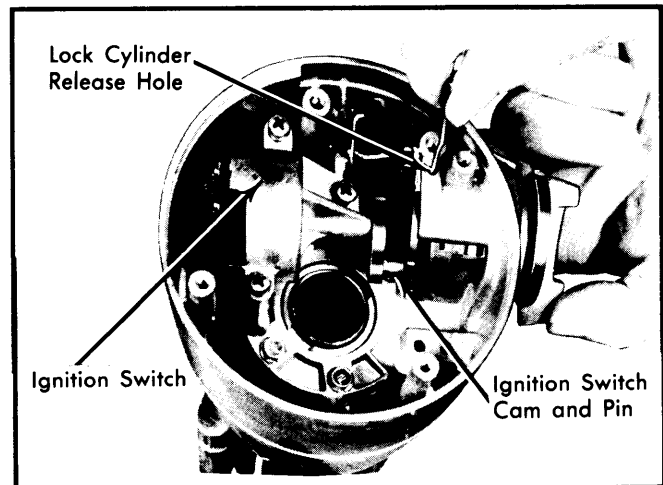
Fig. 4 Depressing Lock Cylinder Retaining Tab Chrysler Corp. Models with Standard Steering Columns
