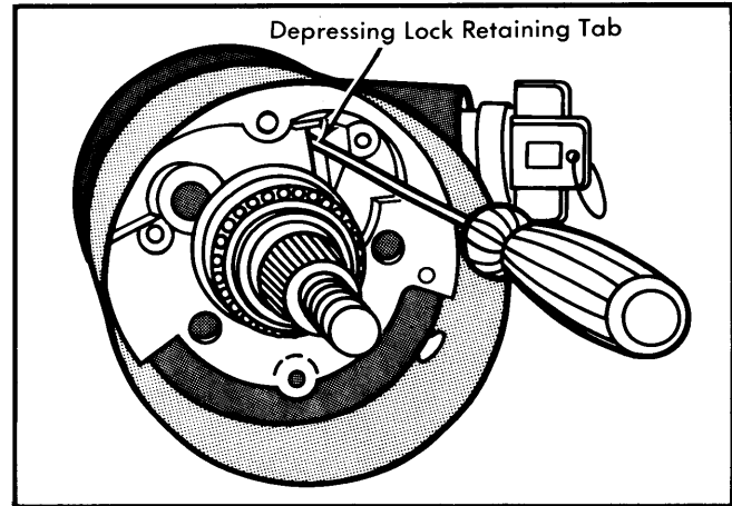
Fig. 3 Depressing Lock Cylinder Retaining Tab on American Motors and General Motors Vehicles
