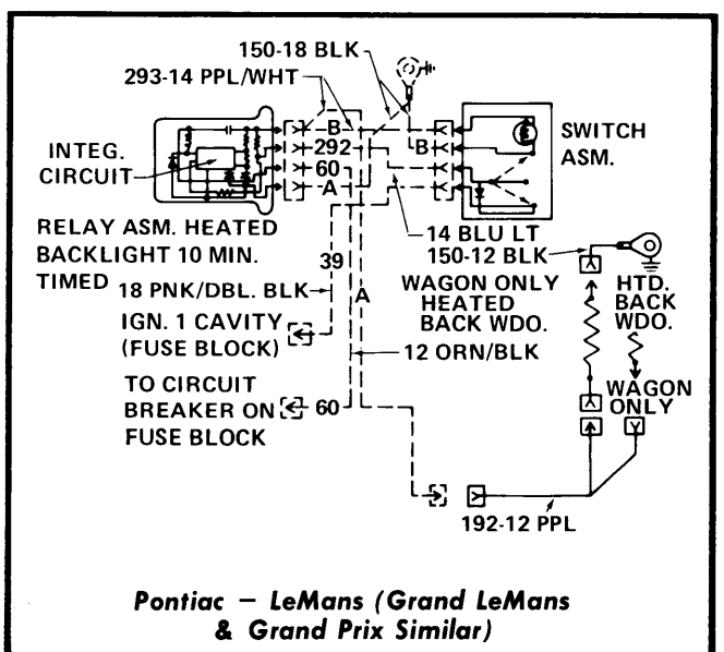
Fig. 3 General Motors Electric Window Defogger Wiring Diagrams
