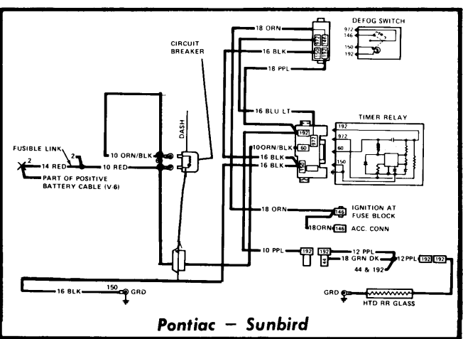
Fig. 3 General Motors Electric Window Defogger Wiring Diagrams
