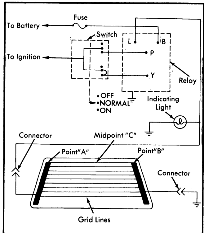
Fig. 3 Chrysler Heated Rear Window Wiring Diagram (Exc. Omni & Horizon)
