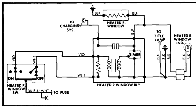
Fig. 4 Omni & Horizon Heated Rear Window Wiring Diagram
