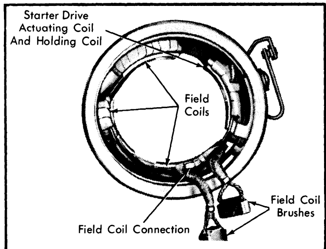
Fig. 4 Field Coil Assembly
