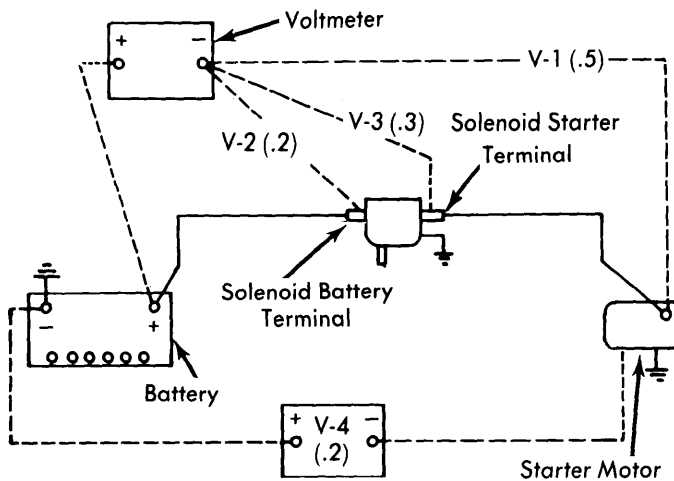
Fig. 1 Starter Cranking Circuit Test Connections
