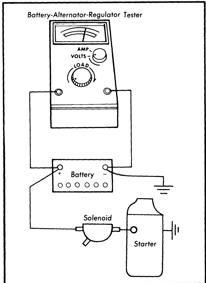
Fig. 2 Starter Load Connections
