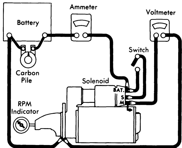
Fig. 2 Starter No Load Connections
