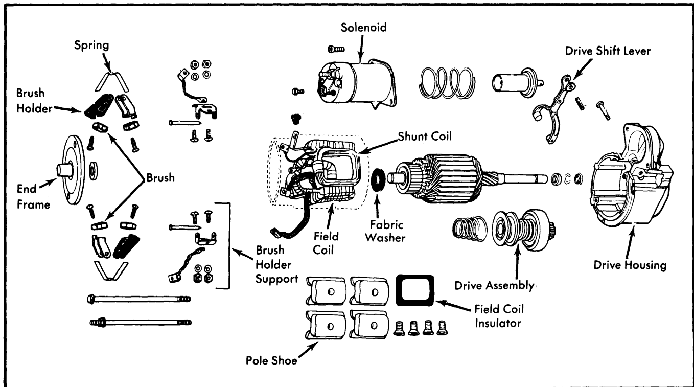
Fig. 4 Exploded View of Starter Motor Assembly — Delco-Remy Enclosed Housing
