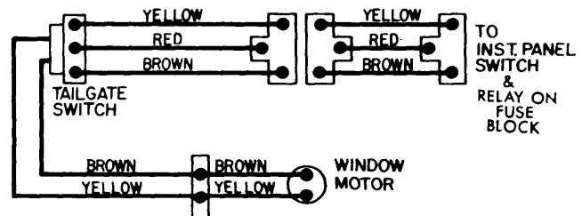
Fig. 1 Chrysler Corp. Tailgate Wiring Diagram
