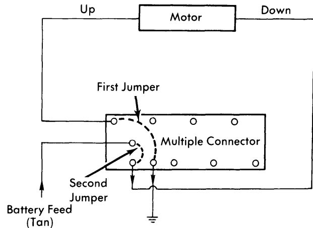
Fig. 2 Switch "DOWN" Test Circuit
