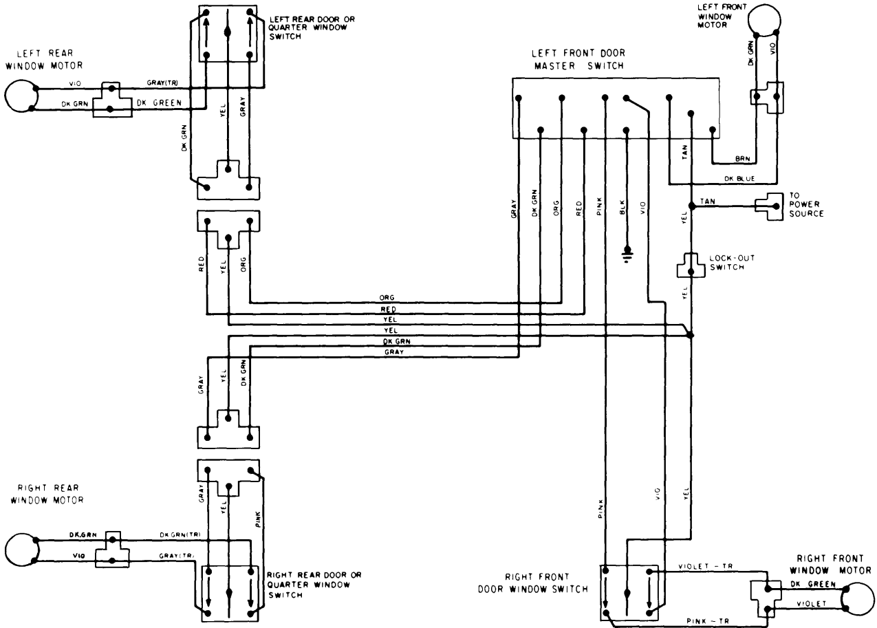
Fig. 3 Chrysler Power Window Wiring Diagram
