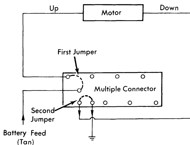
Fig. 1 Switch "UP" Test Circuit
