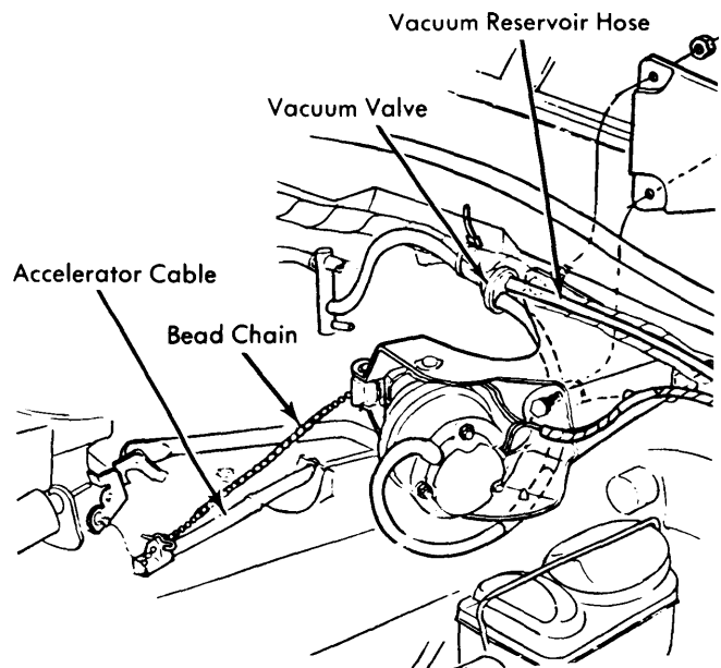
Fig. 3 Engine Compartment Speed Control Components for Thunderbird, LTD II, and Cougar with 351 and 400 Engines
