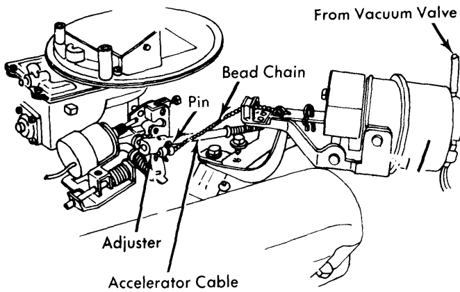
Fig. 4 Engine Compartment Speed Control Components for Granada and Monarch V8 (Thunderbird, LTD II, and Cougar with 302" Engine is Similar)
