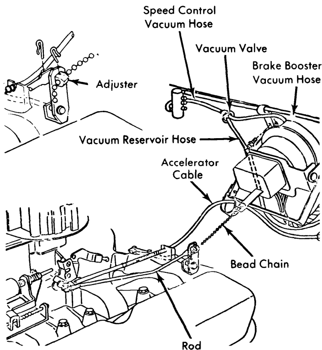
Fig. 2 Engine Compartment Speed Control Components for Ford and Mercury Models
