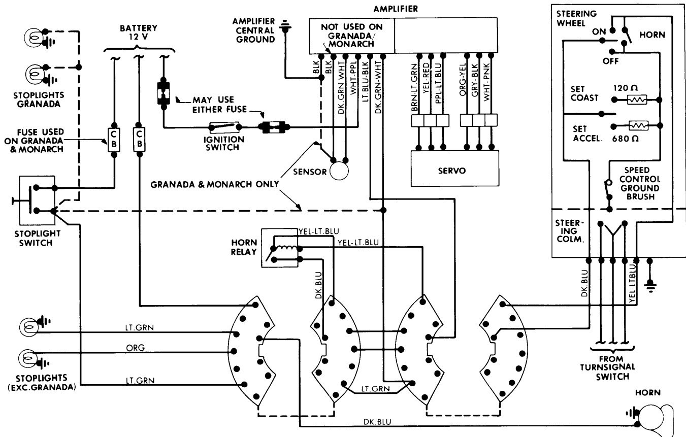
Fig. 1 Wiring Diagram of Ford Motor Co. Automatic Speed Control System.
