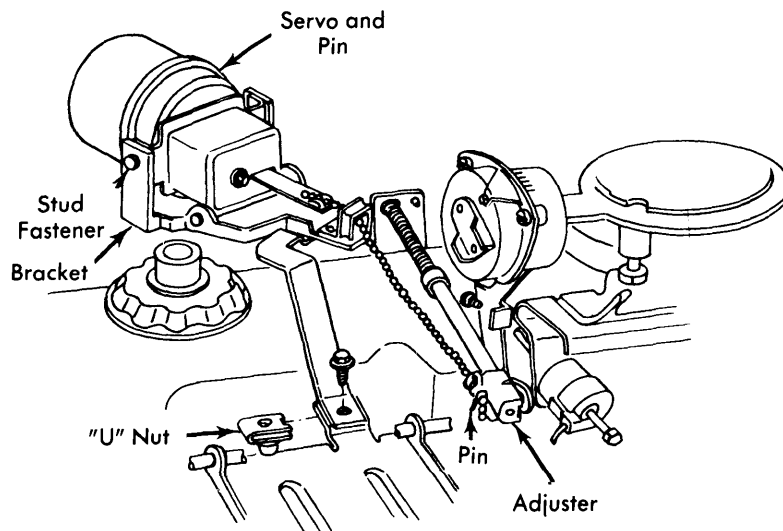
Fig. 6 Engine Compartment Speed Control Components for Granada and Monarch Six Cylinder Engine
