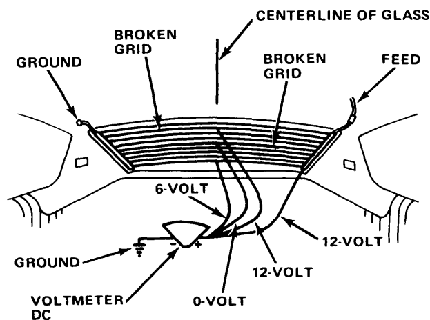
Fig. 3 Testing Gremlin, Hornet and Matador Window Grids Using Voltmeter By Checking Voltage Drop for Grid Continuity
