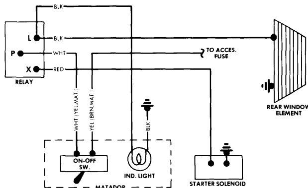
Fig. 1 American Motors Heated Rear Window Wiring
