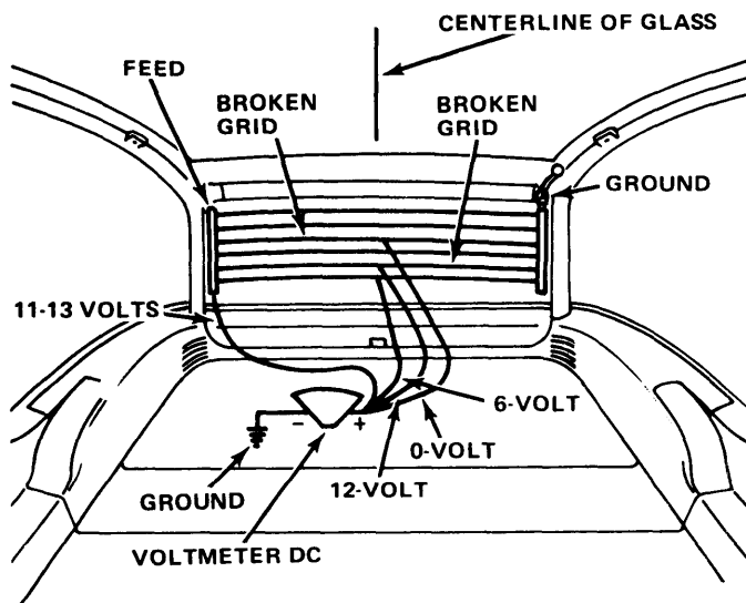
Fig. 2 Testing Pacer Window Grids Using Voltmeter By Checking Voltage Drop for Grid Continuity
