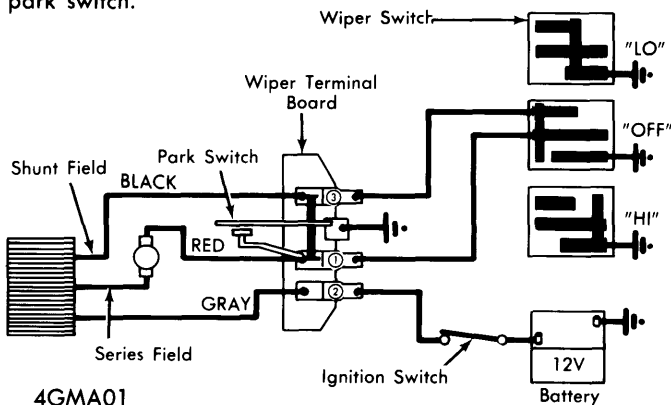
WIPER SYSTEM WIRING DIAGRAM
