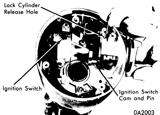
TYPICAL CHRYSLER IGNITION SWITCH AND LOCK (STANDARD COLUMN)
