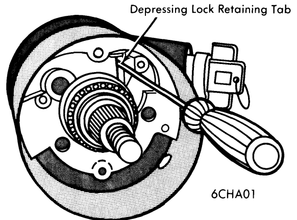
LOCK CYLINDER REMOVAL (AMC & GENERAL MOTORS)
