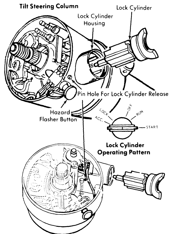
Fixed Steering Column
