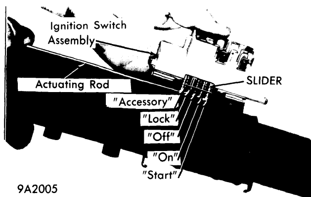
TYPICAL IGNITION SWITCH (EXC. CHRYSLER STANDARD COLUMN)
