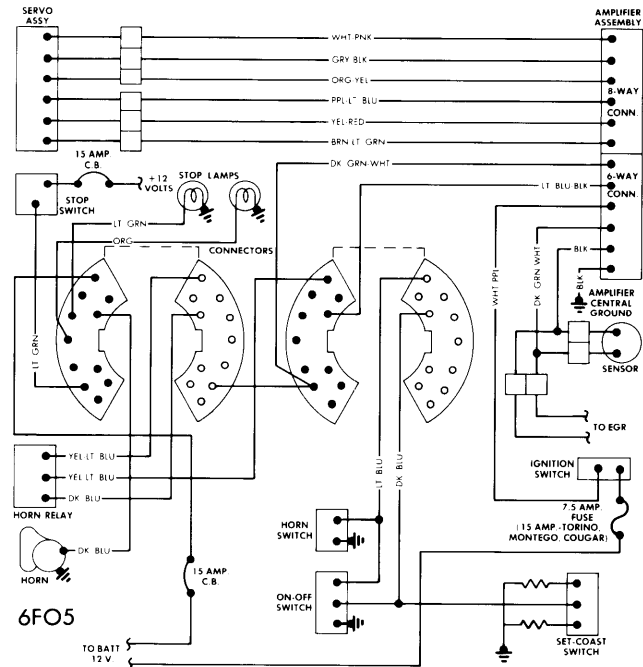
FORD MOTOR CO. SPEED CONTROL WIRING (EXC. GRANADA, MONARCH, THUNDERBIRD, LINCOLN & MARK IV)
