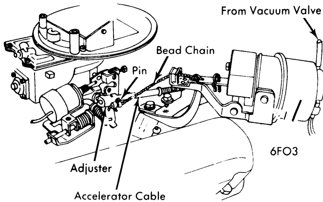
SPEED CONTROL SENSOR & SERVO (GRANADA & MONARCH - V8 SHOWN)
