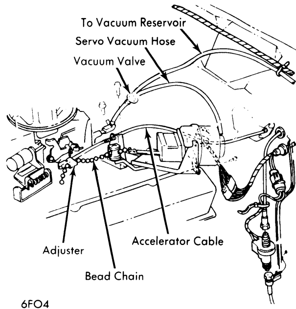
SPEED CONTROL SENSOR & SERVO (THUNDERBIRD, LINCOLN, & MARK IV)
