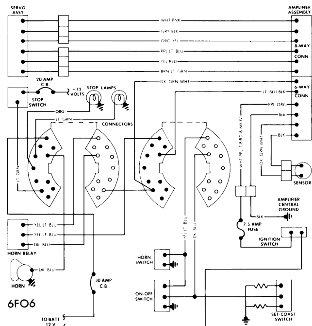
FORD MOTOR CO. SPEED CONTROL WIRING (THUNDERBIRD, LINCOLN & MARK IV)
