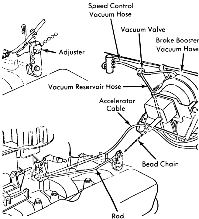
SPEED CONTROL SENSOR & SERVO (FORD & MERCURY)
