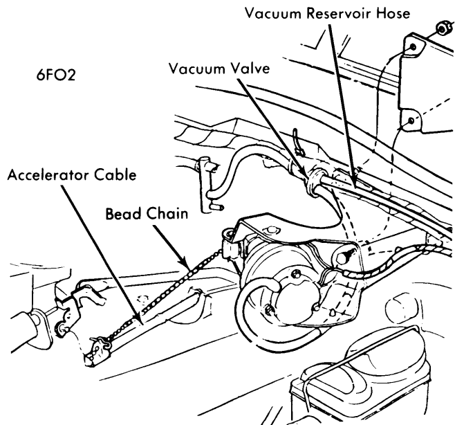
SPEED CONTROL SENSOR & SERVO (TORINO, MONTEGO, ELITE & COUGAR)
