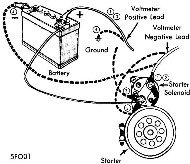
5FO01 CRANKING CIRCUIT TEST CONNECTIONS
