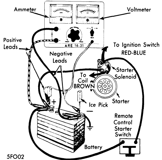
5FO02 STARTER LOAD TEST CONNECTIONS
