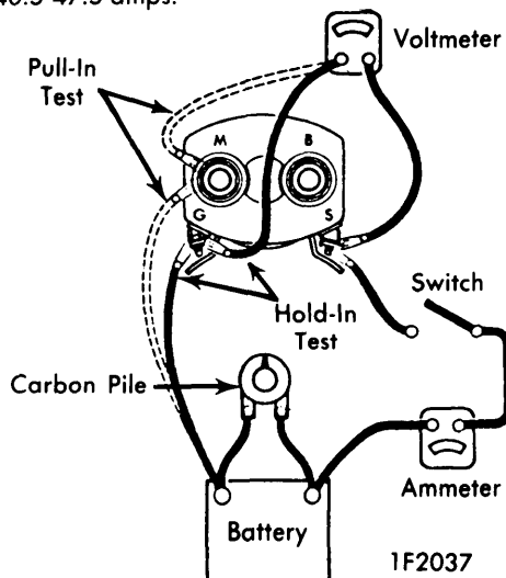
SOLENOID WINDING TEST CONNECTIONS
