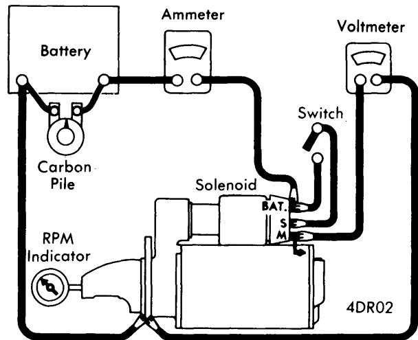
STARTER NO LOAD TEST CONNECTIONS
